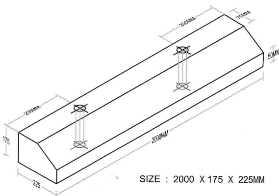
ISOMETRIC VIEW
